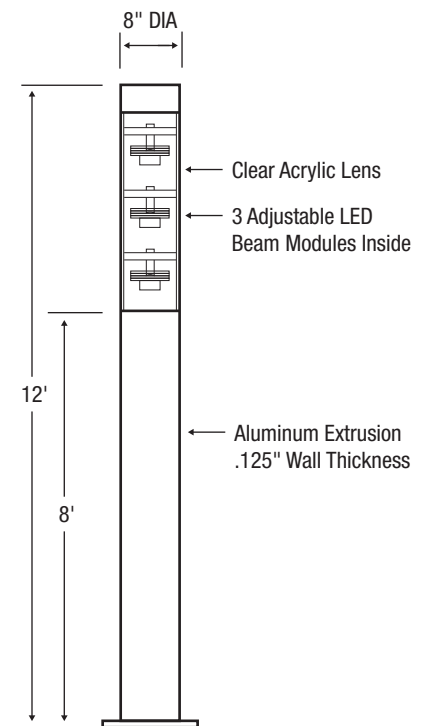
LED 60° Light Beam Module with Rotation (350°) and Horizontal (80°) Adjustment
